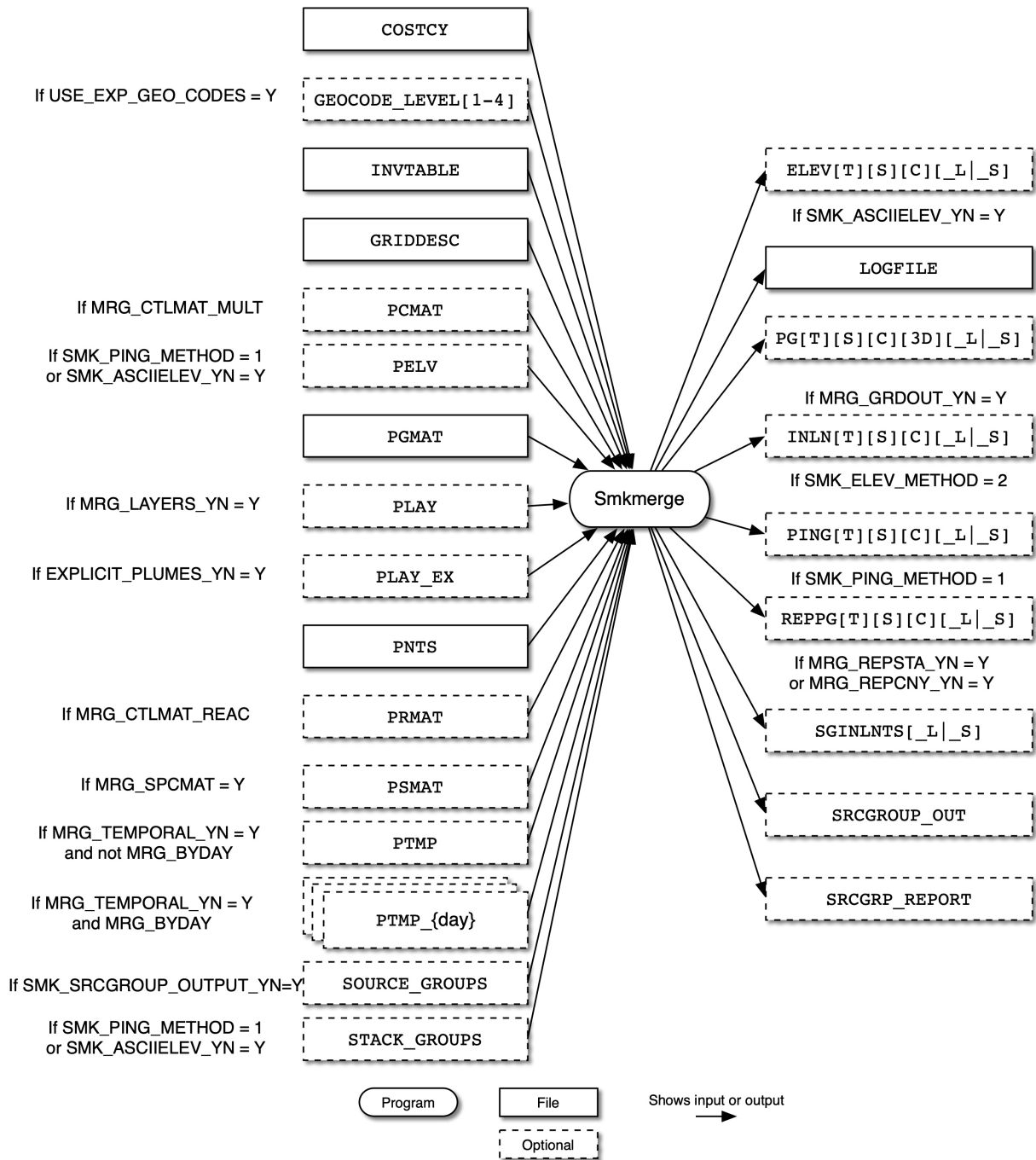
Figure 4.24, “ Smkmerge input and output files for point sources” [196] shows the input and output files for the Smkmerge program for point sources. The inputs include the country, state, and county codes file ( COSTCY ), the inventory data table ( INVTABLE ), the grid description file ( GRIDDESC ), and the optional multiplicative control matrix from Cntlmat ( PCMAT ). If using PinG or elevated sources, the PELV file is used. Smkmerge reads the gridding matrix output from Grdmat ( PGMAT ). The PLAY file is used to merge layer fractions, while the PLAY_EX file is used for explicit plumes. Other Smkmerge input files include the inventory file output from Smkinven ( PNTS ), the optional reactivity matrix from Cntlmat ( PRMAT ), and the optional speciation matrix from Spmat ( PSMAT ). The hourly emissions from Temporal are
