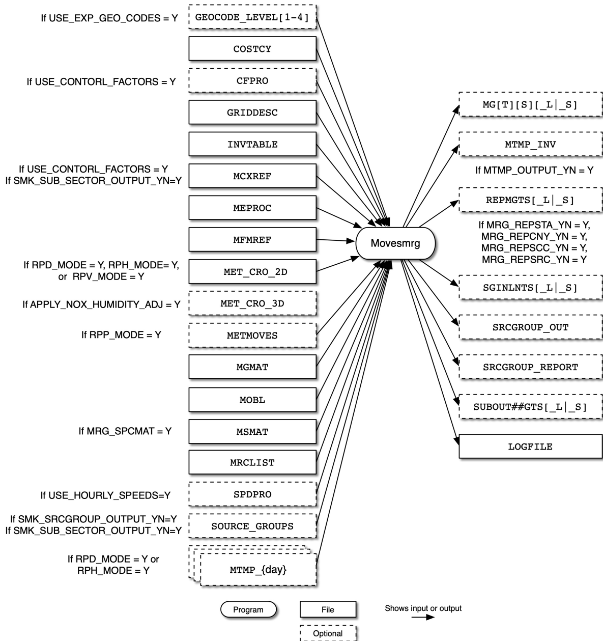
Figure 4.8, “ Movesmrg input and output files” [160] shows the input and output files for the Movesmrg program. The input files are the country, state, and county codes file ( COSTCY ), the grid description file ( GRIDDESC ), the inventory data table ( INVTABLE ), the representative county fuel month file ( MFMREF ), the list of emission process and associated pollutants file ( MEPROC ), the representative county cross-reference file ( MCXREF ), the list of emission factors files by representative county file ( MRCLIST ), the meteorology files ( MET_CRO_2D ), the gridding matrix from Grdmat ( MGMAT ), the inventory file output from Smkinven ( MOBL ), the speciation matrix from Spcmat ( MSMAT_L or MSMAT_S ), the Met4moves output file for
