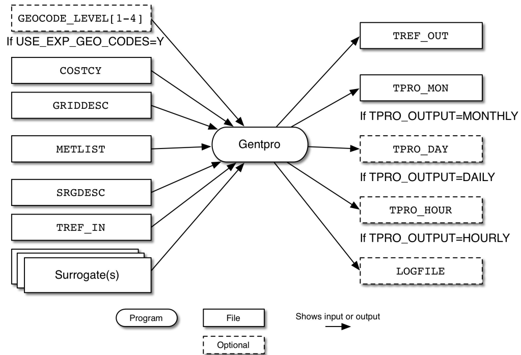
Figure 3.1. Gentpro input and output files
