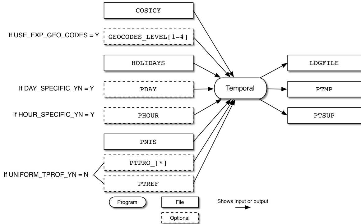
Figure 4.29. Temporal input and output files for point sources
