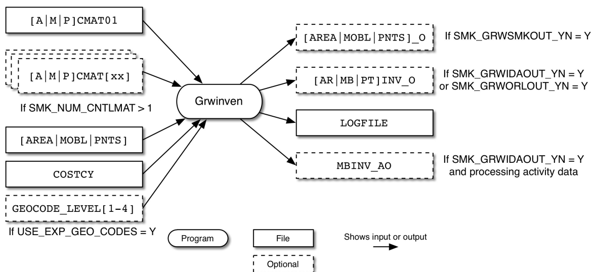
Figure 4.5. Grwinven input and output files
