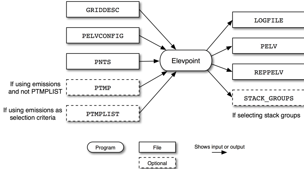
Figure 4.3. Elevpoint input and output files
