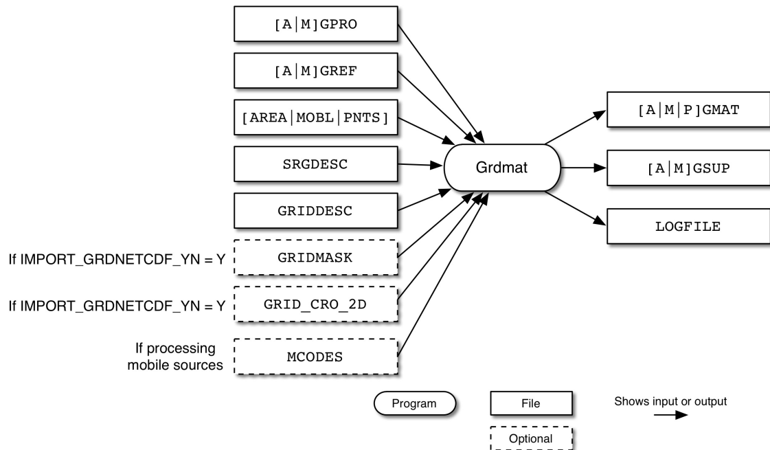
Figure 4.4, “ Grdmat input and output files” [146] shows the input and output files for the Grdmat program. The input files are the spatial surrogates file (AGPRO or MGPRO), the spatial cross-reference file (AGREF
