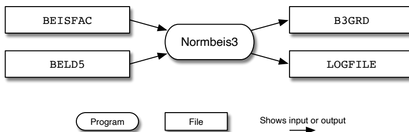
Figure 4.14. Normbeis3 input and output files for BEIS v3.7 or later version
