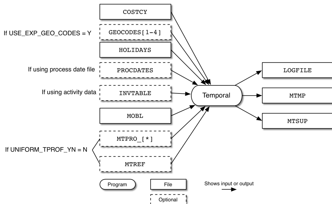
Figure 6.25. Temporal input and output files for mobile sources
