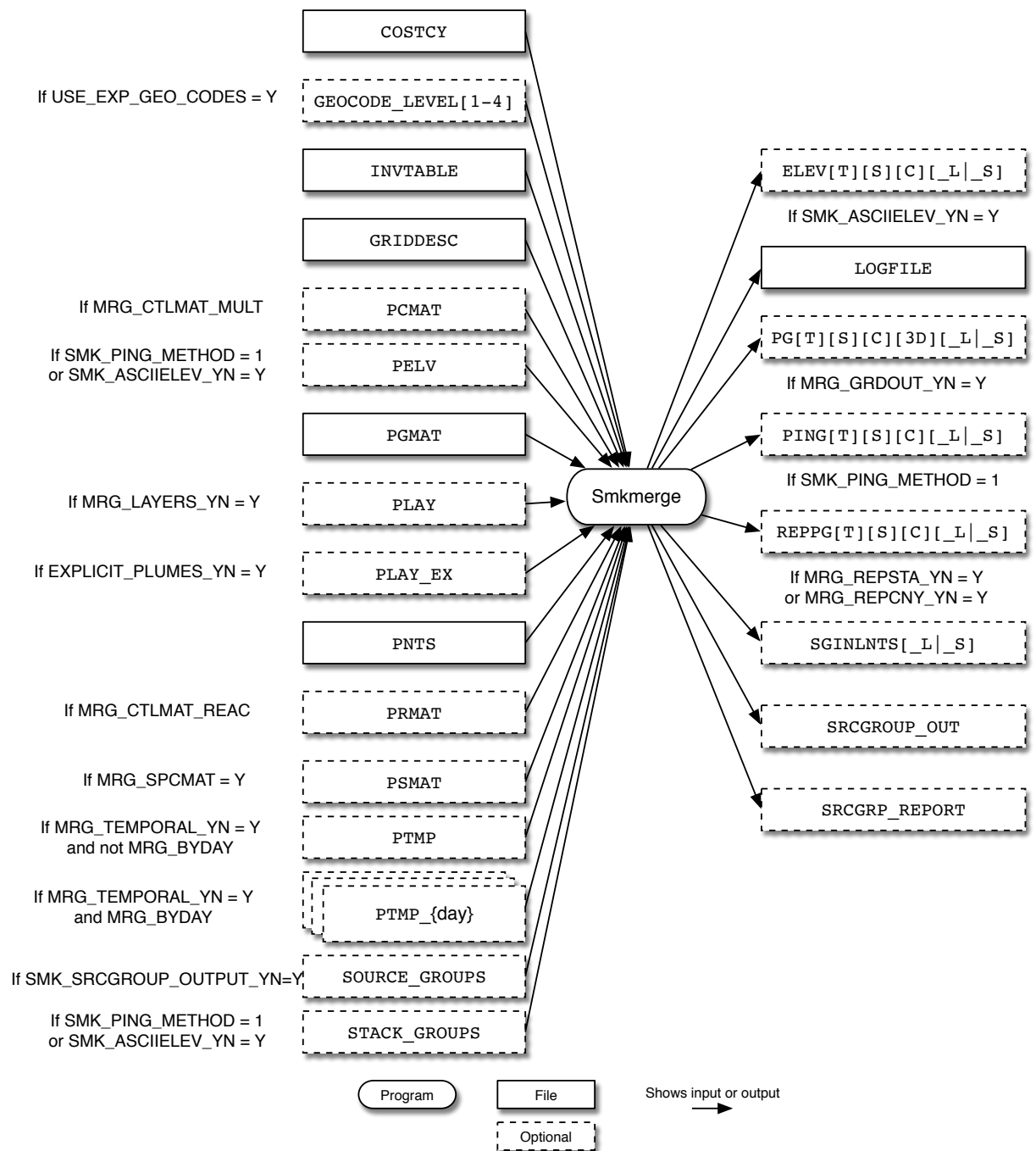
Figure 6.21. Smkmerge input and output files for point sources
