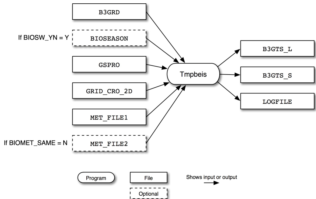
Figure 6.27. Tmpbeis3 input and output files
