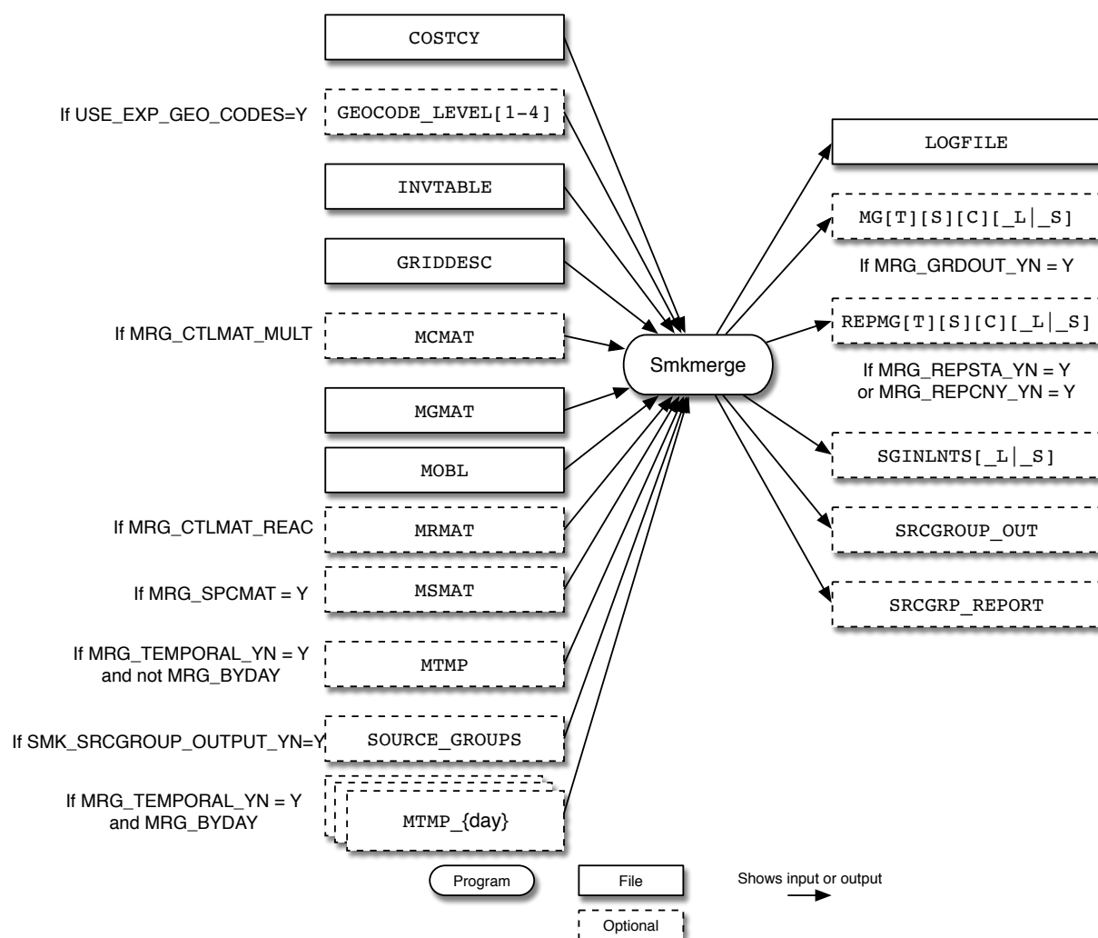
Figure 6.20. Smkmerge input and output files for mobile sources
