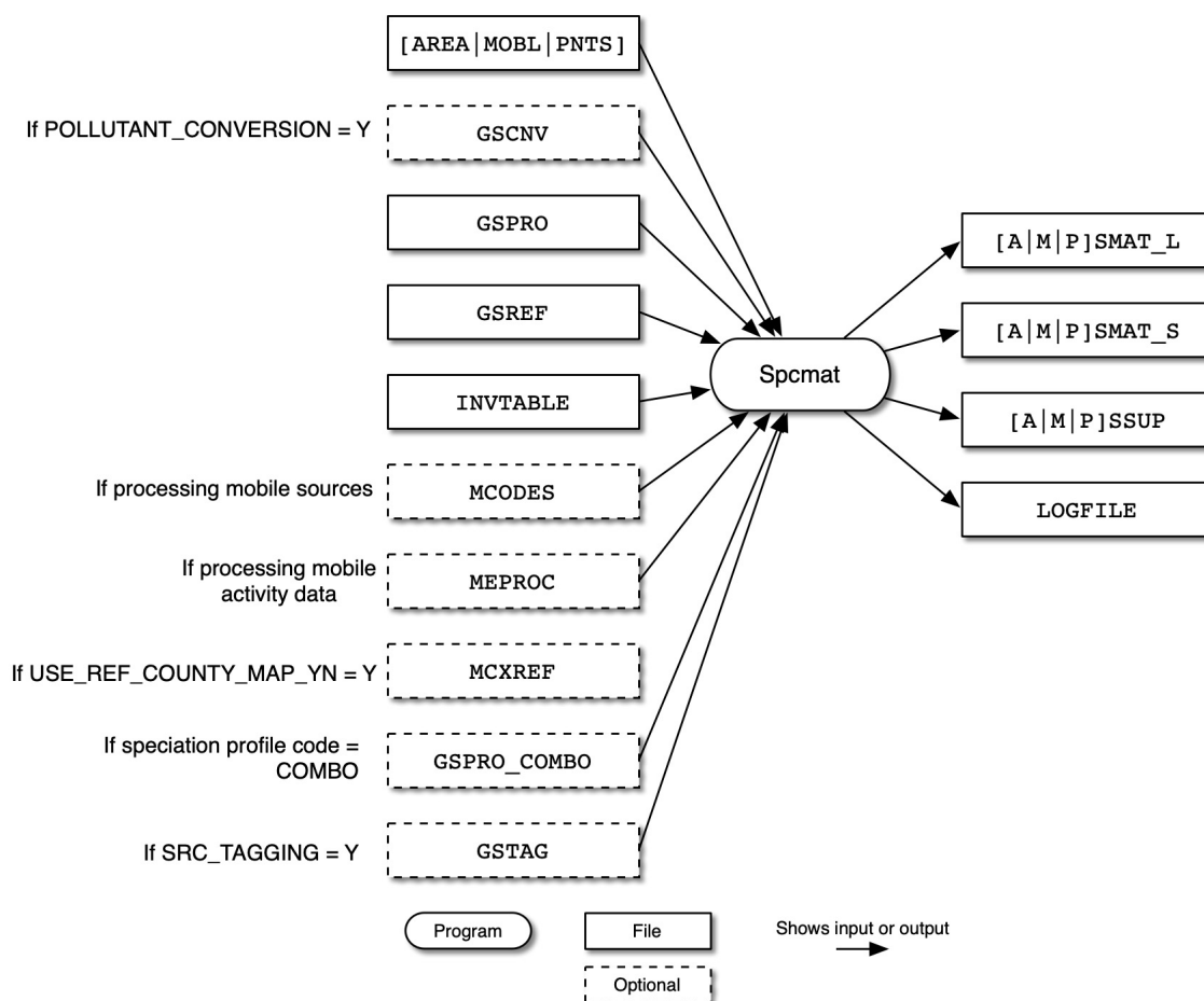
Figure 6.23. Spcmat input and output files
