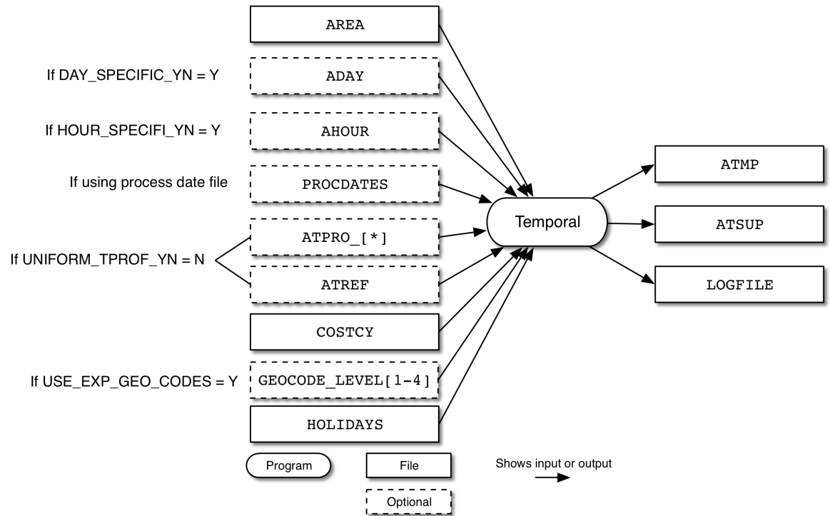
Figure 6.24. Temporal input and output files for area sources
