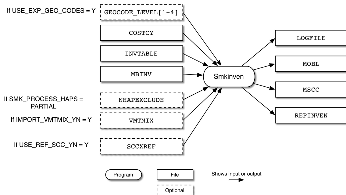
Figure 6.16. Smkinven input and output files for mobile sources
