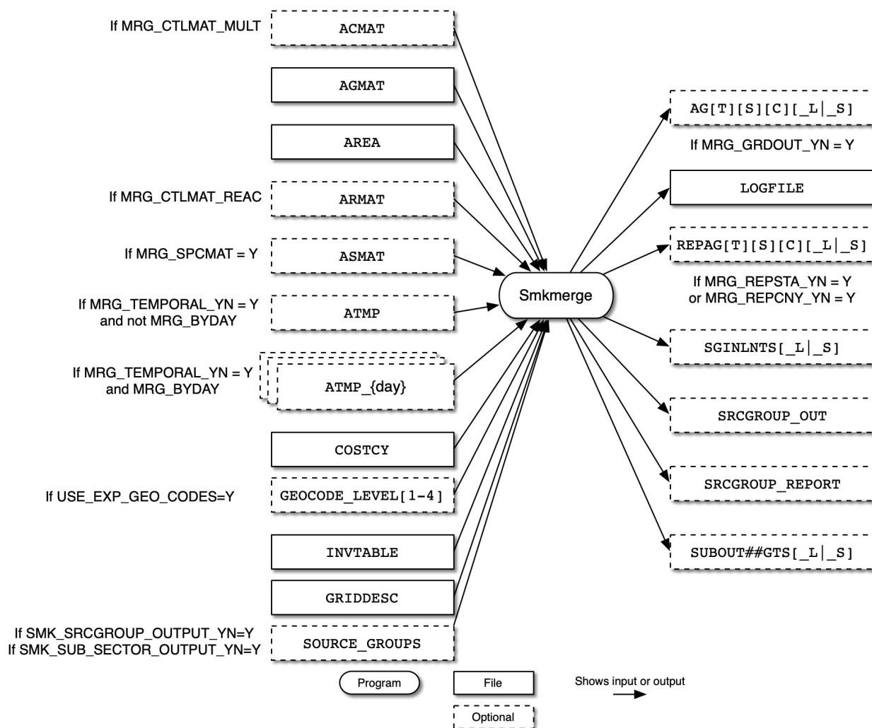
Figure 6.18. Smkmerge input and output files for area sources
