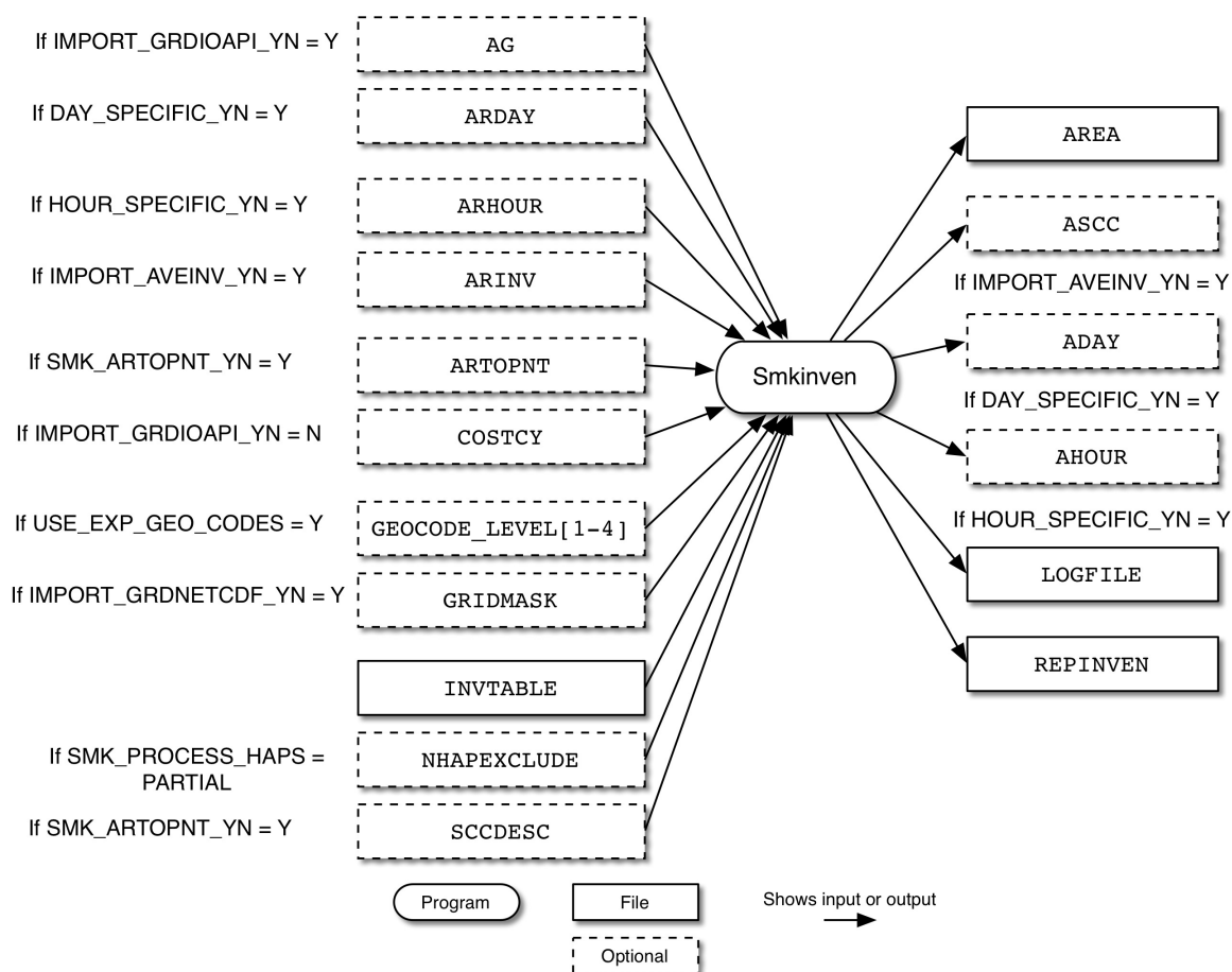
Figure 6.15. Smkinven input and output files for area sources
