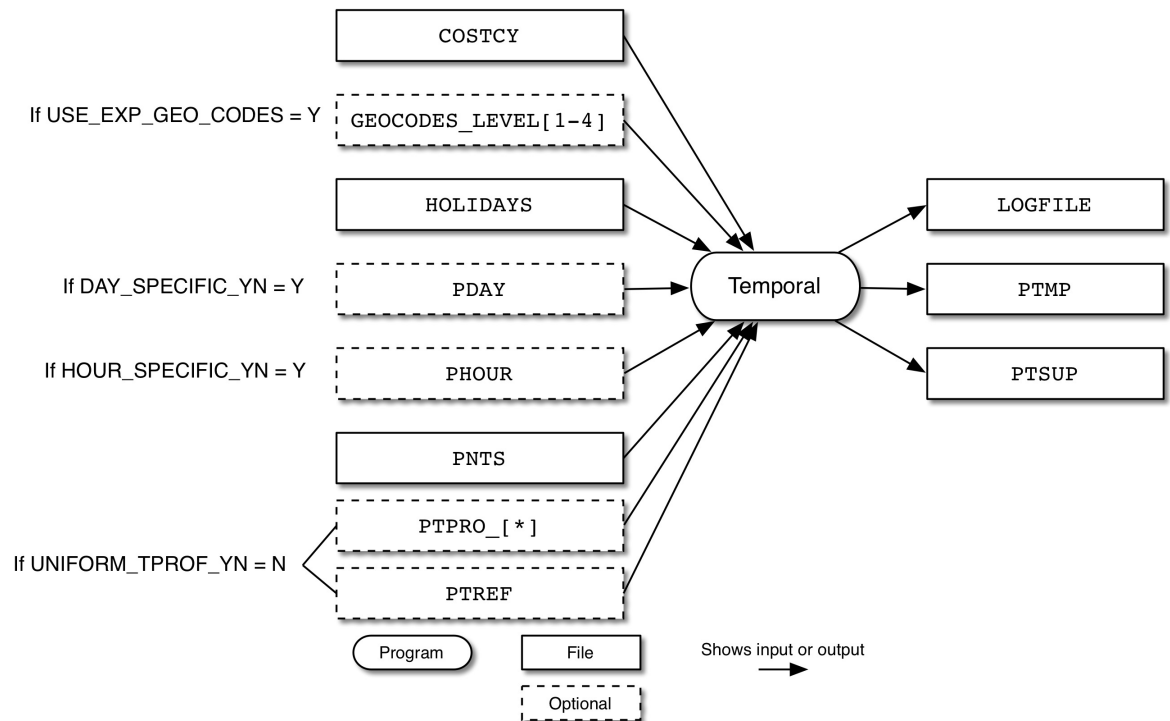
Figure 6.26. Temporal input and output files for point sources
