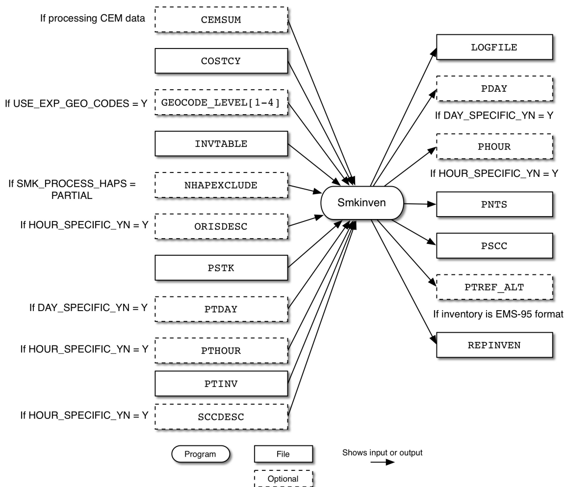
Figure 6.17. Smkinven input and output files for point sources
