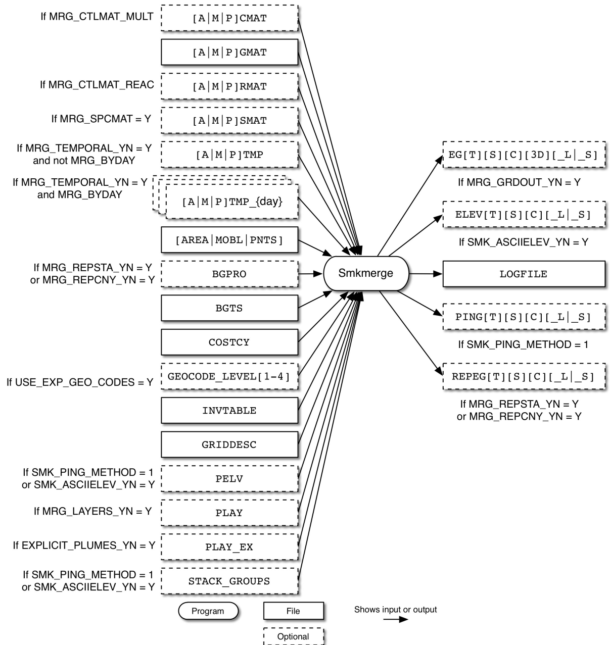
Figure 6.22. Smkmerge input and output files for all source categories
