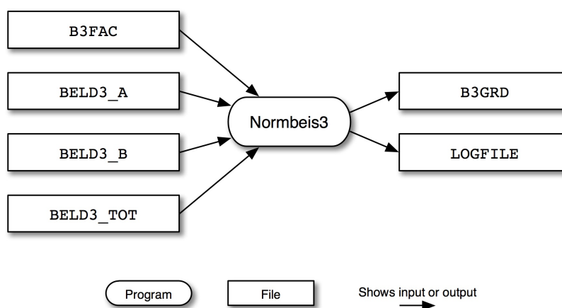
Figure 6.12. Normbeis3 input and output files
