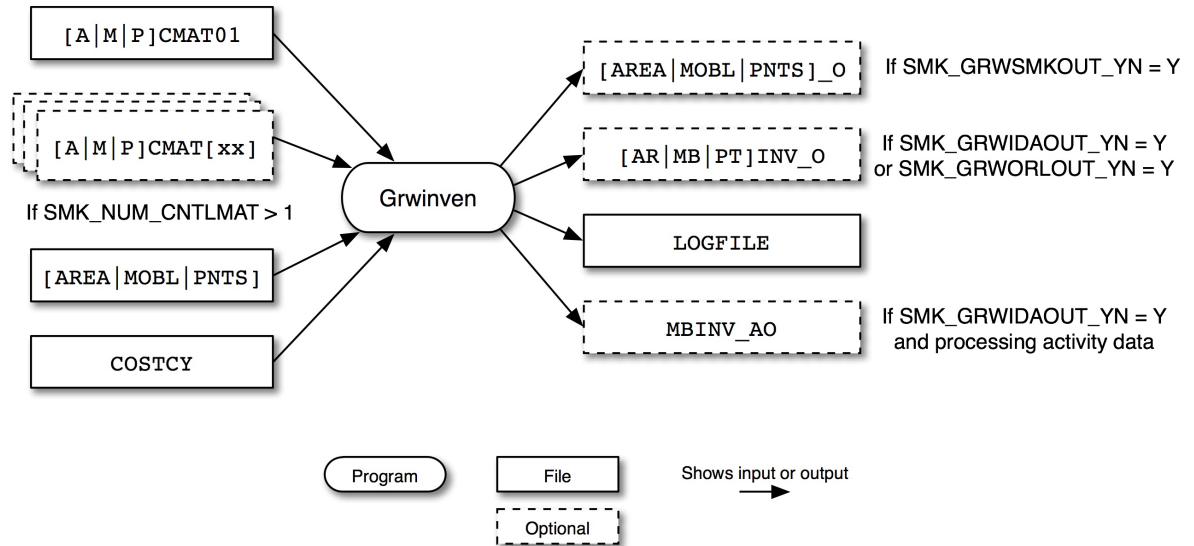
Figure 6.5. Grwinven input and output files
