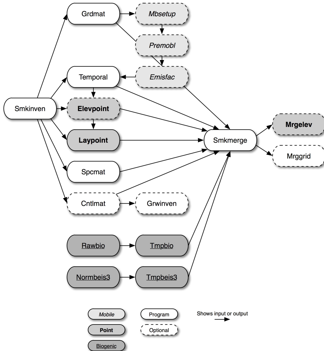
Figure 6.1. SMOKE core programs
