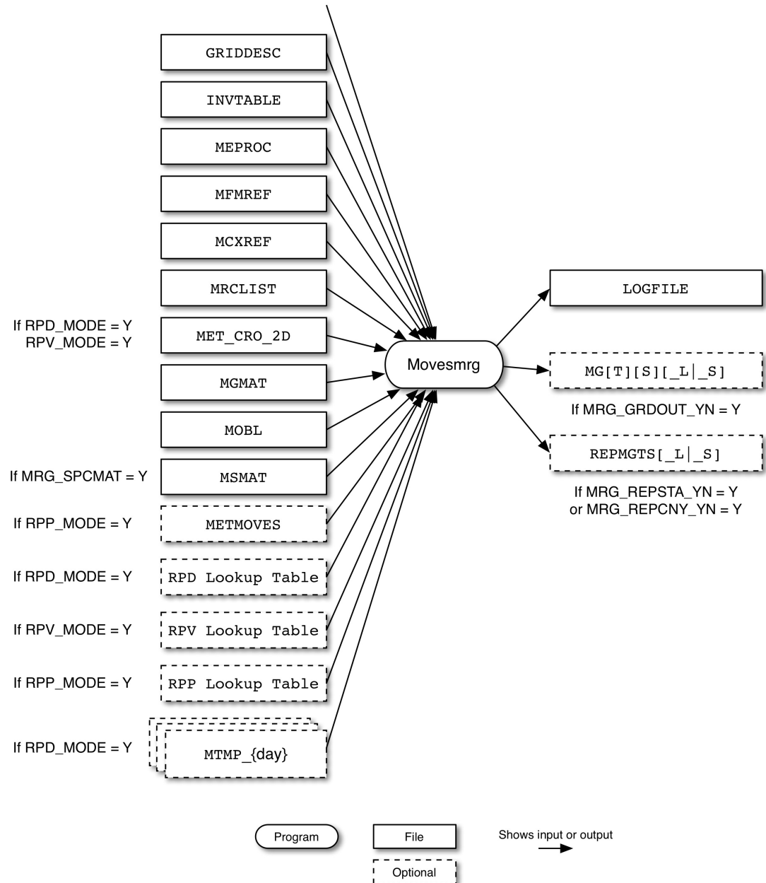
Figure 6.10. Movesmrg input and output files
