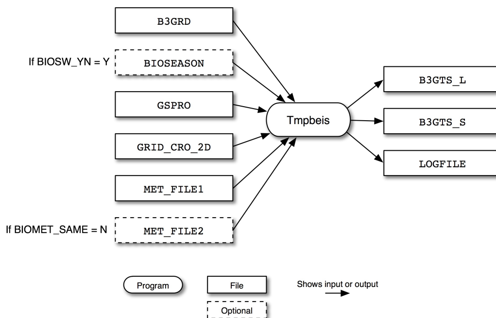
Figure 6.28. Tmpbeis3 input and output files
