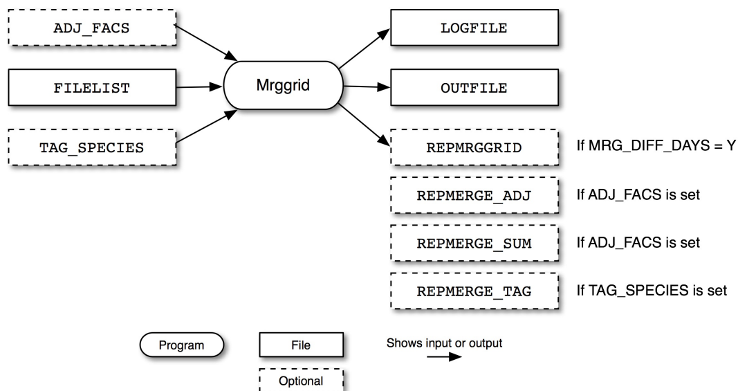
Figure 6.12. Mrgrid input and output files
