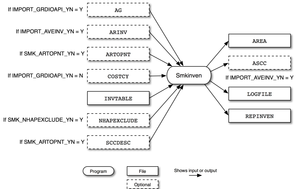
Figure 6.16. Smkinven input and output files for area sources
