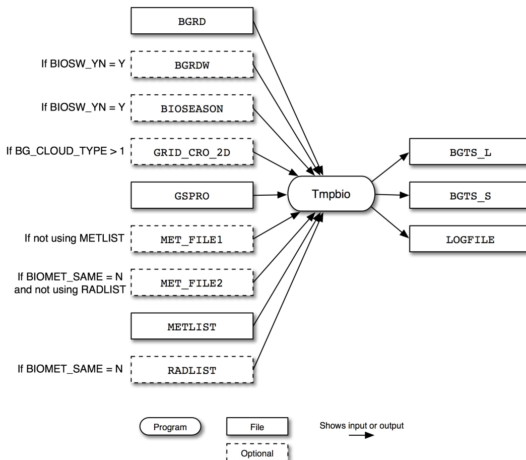
Figure 6.29. Tmpbio input and output files
