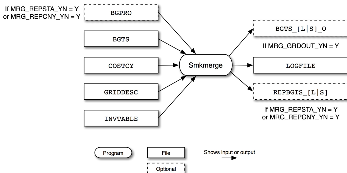
Figure 6.20. Smkmerge input and output files for biogenic sources
