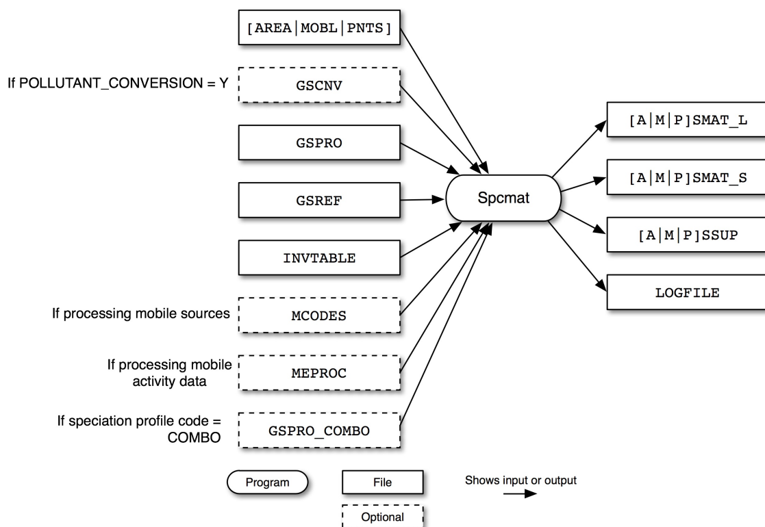
Figure 6.24. Spcmat input and output files
