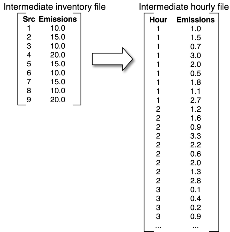
Figure 2.22. Transformation of inventory data to hourly data
