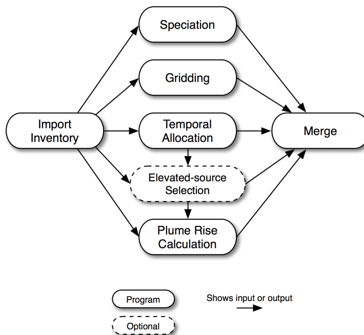
Figure 2.17. Base case point-source processing steps for the CMAQ-based approach
