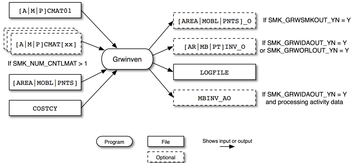
Figure 6.6. Grwinven input and output files
