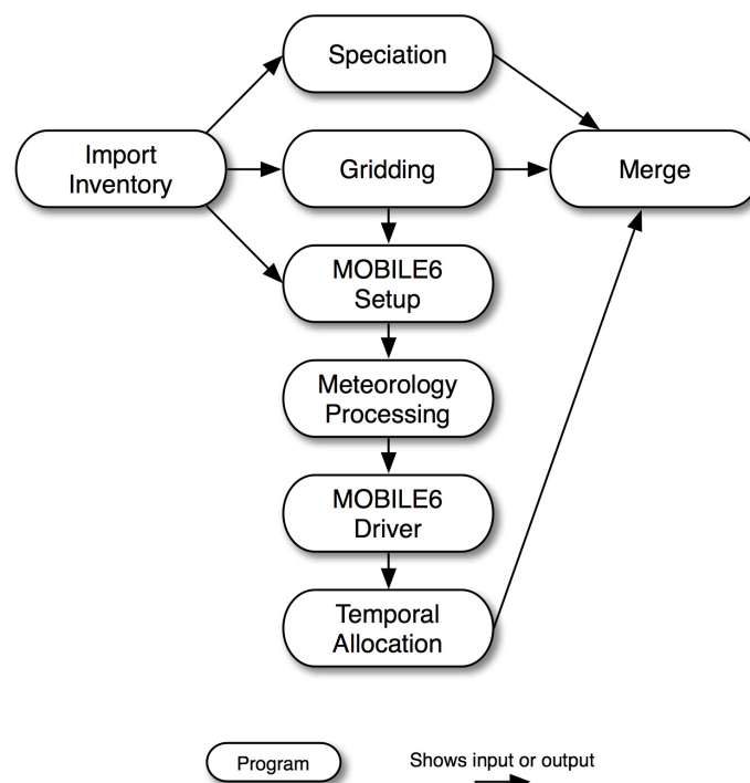
Figure 2.13. Base case mobile VMT approach processing steps
