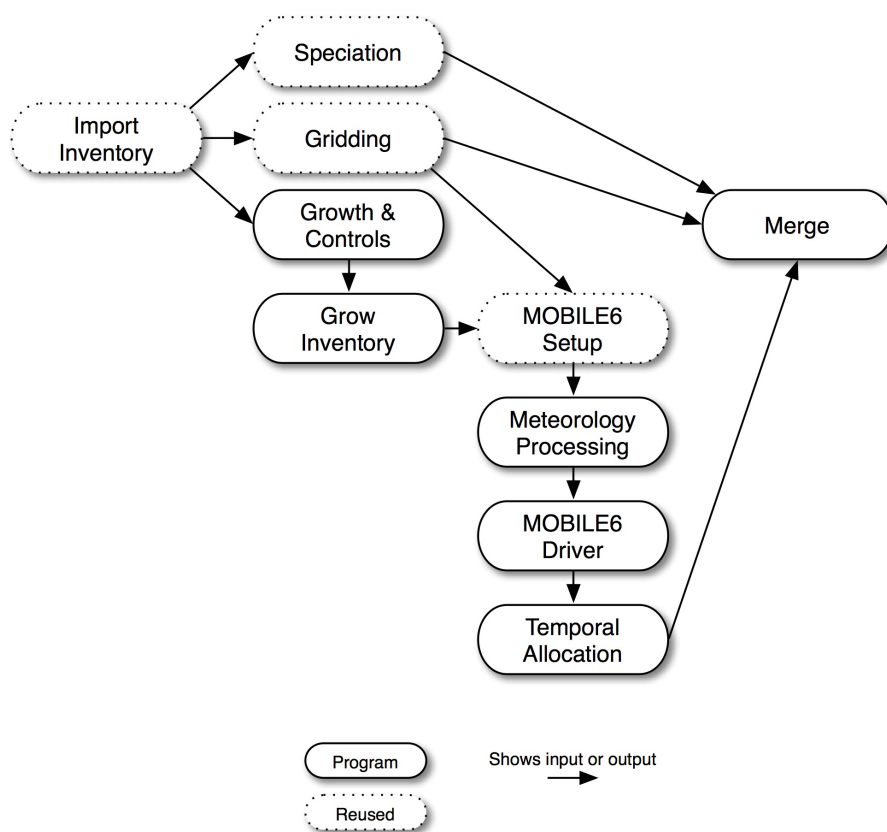
Figure 2.14. Future- or past-year growth and control mobile-source processing steps
