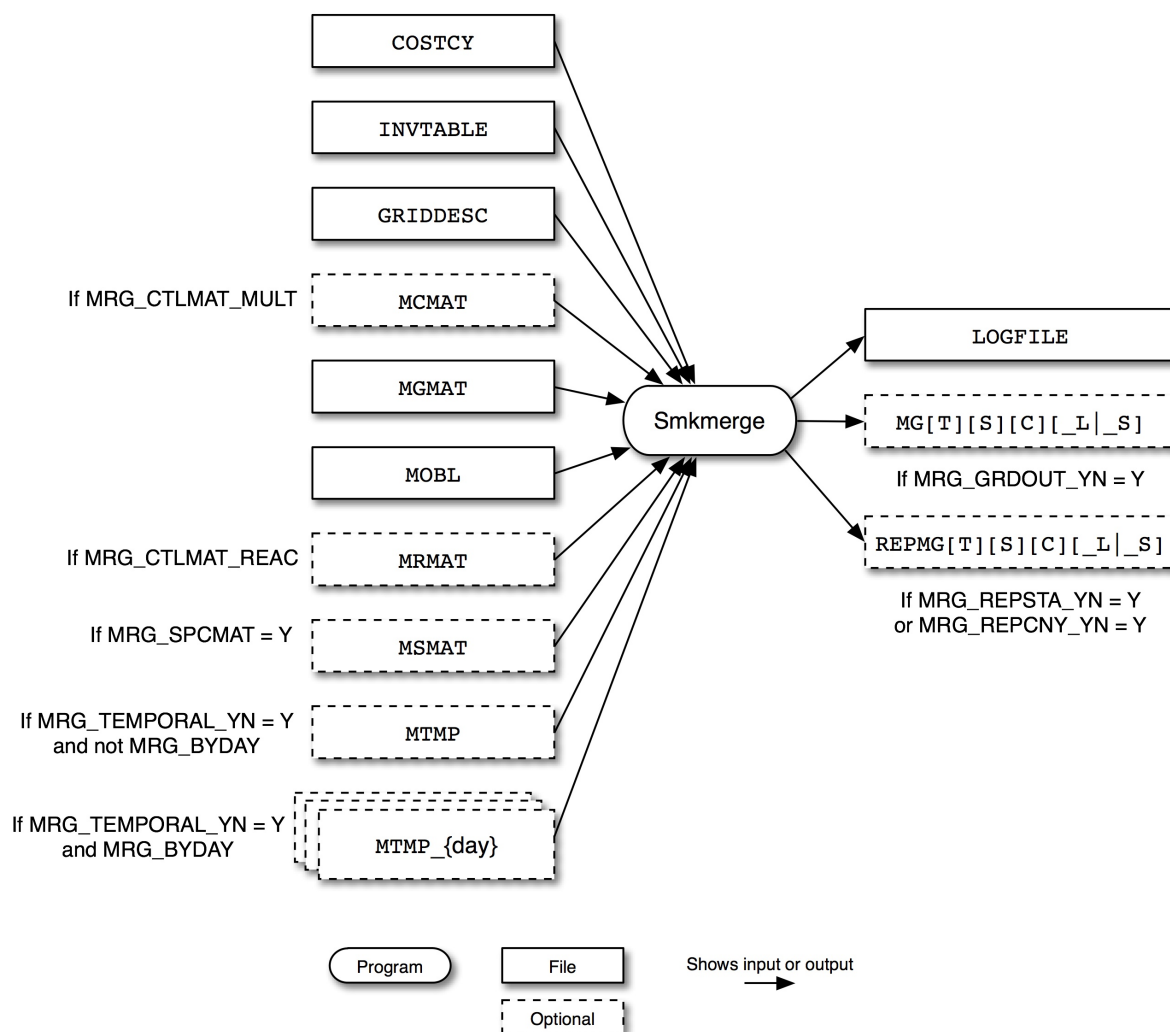
Figure 6.21. Smkmerge input and output files for mobile sources
