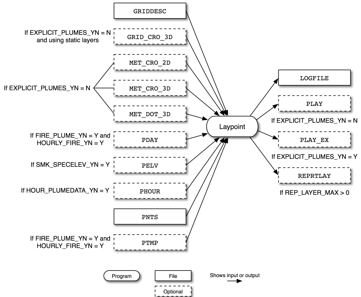
Figure 6.7. Laypoint input and output files
