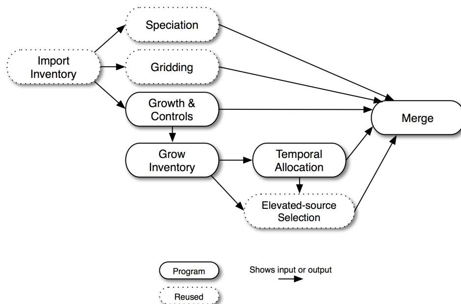
Figure 2.20. Future- or past-year growth and control point-source processing steps for the UAM-based approach
