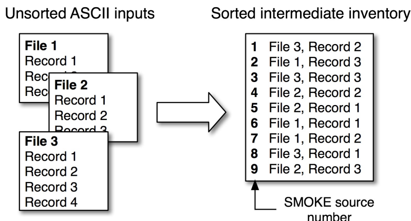
Figure 2.21. Combining and sorting ASCII inputs to created sorted I/O API outputs
