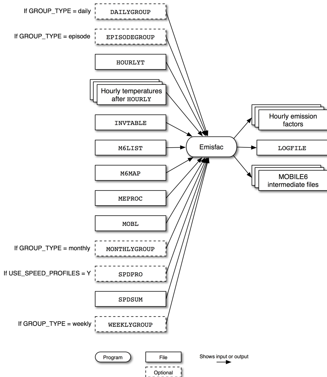
Figure 6.4. Emisfac input and output files
