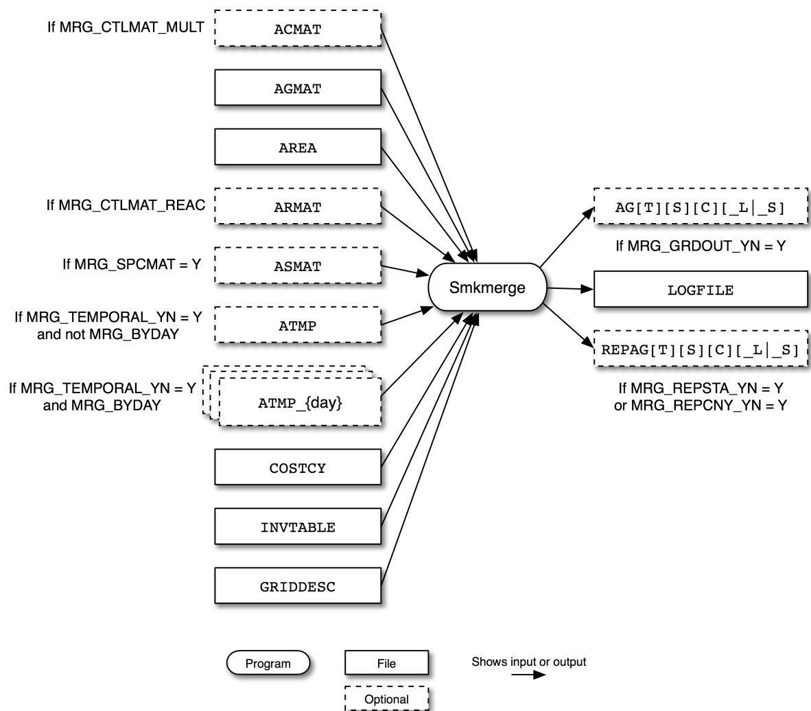
Figure 6.19. Smkmerge input and output files for area sources
