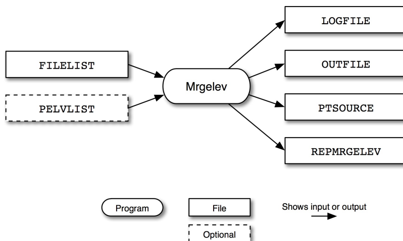
Figure 6.11. Mrgelev input and output files
