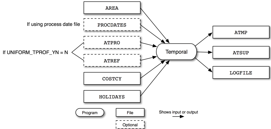
Figure 6.25. Temporal input and output files for area sources
