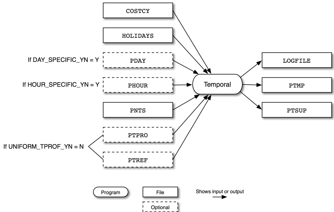
Figure 6.27. Temporal input and output files for point sources
