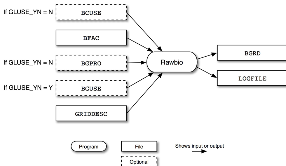
Figure 6.15. Rawbio input and output files
