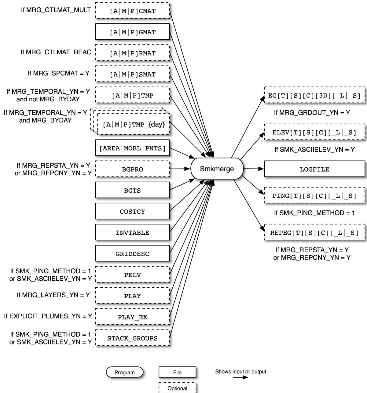
Figure 6.23. Smkmerge input and output files for all source categories
