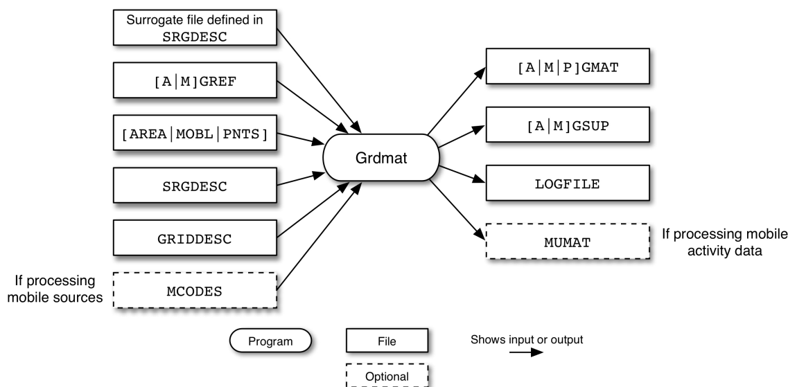
Figure 6.5. Grdmat input and output files
