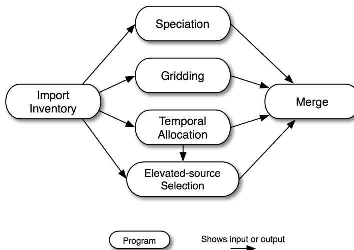
Figure 2.18. Base case point-source processing steps for the UAM-based approach
