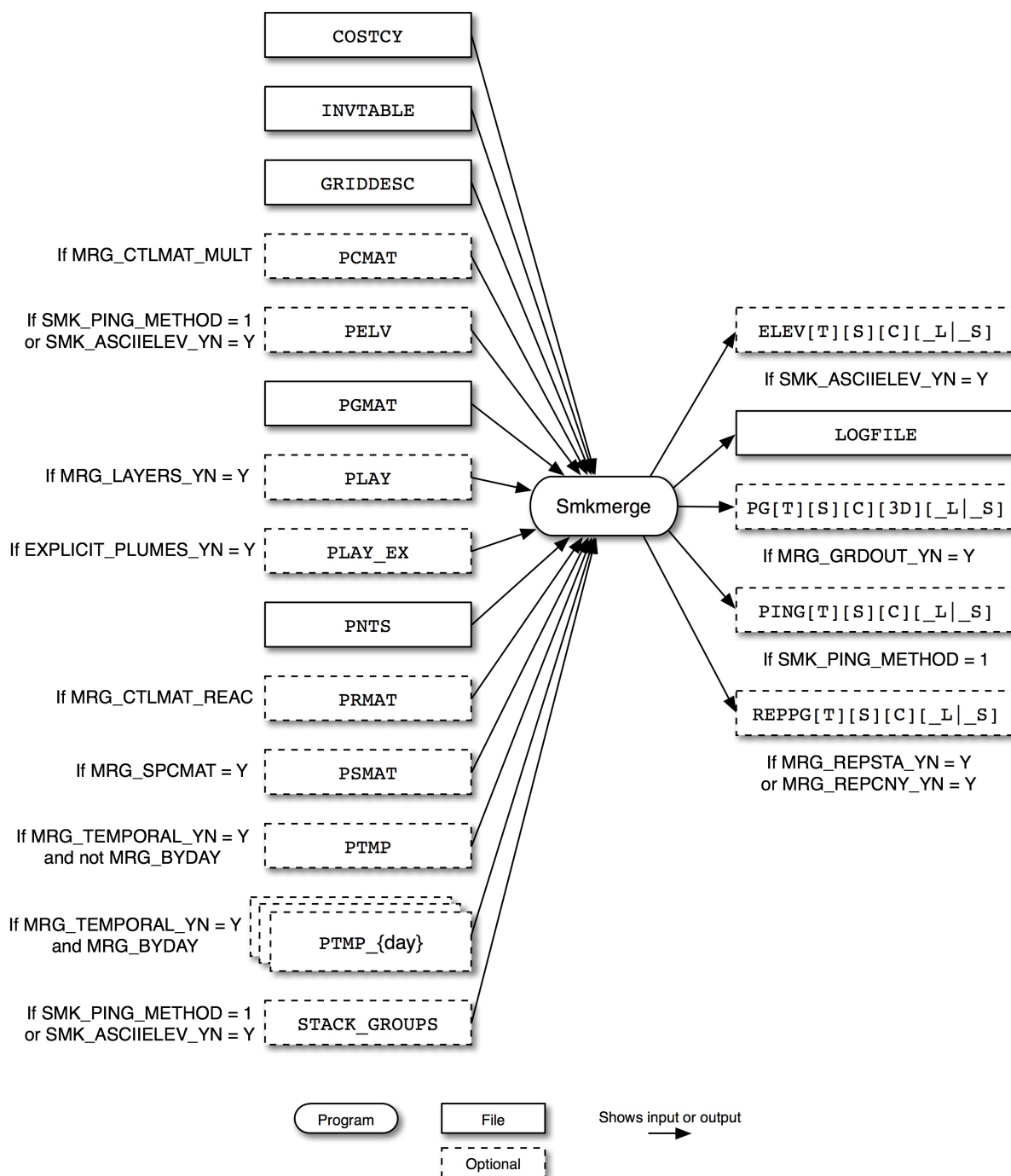
Figure 6.22. Smkmerge input and output files for point sources
