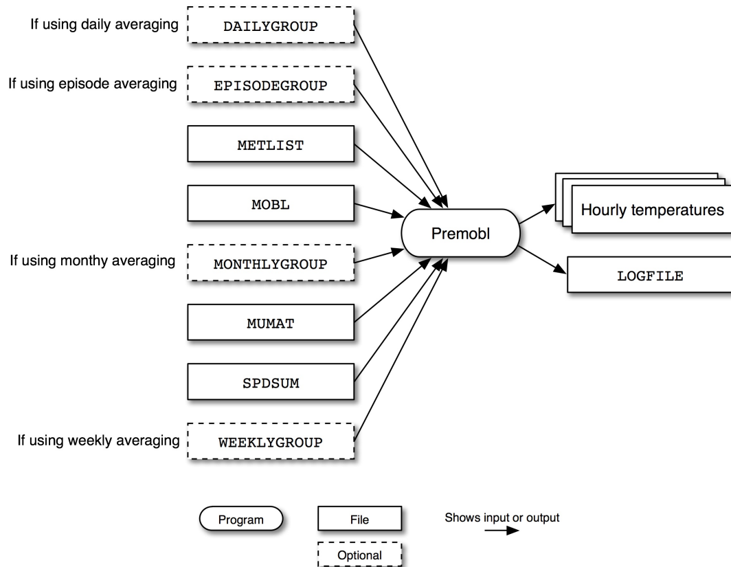
Figure 6.14. Premobl input and output files
