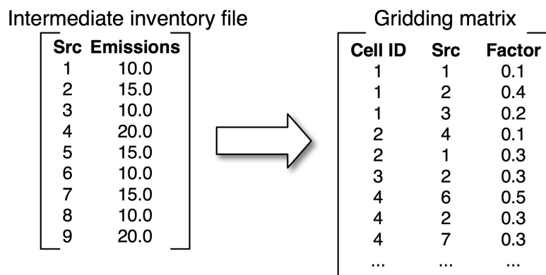
Figure 2.24. Relationship between inventory and gridding matrix
