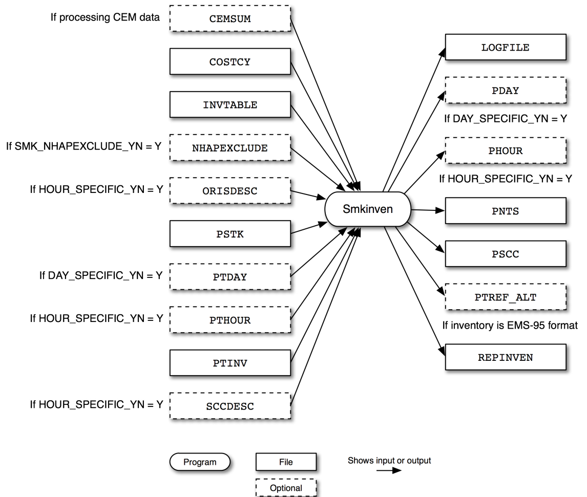
Figure 6.18. Smkinven input and output files for point sources
