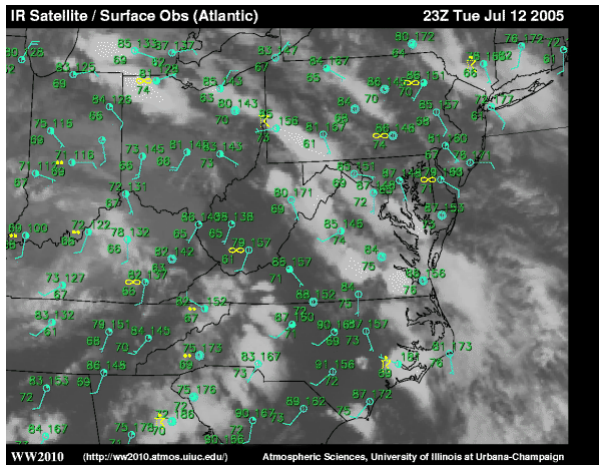
Fig. 6. Surface observations for Tuesday, July 12, 2005, 2300 UTC.
