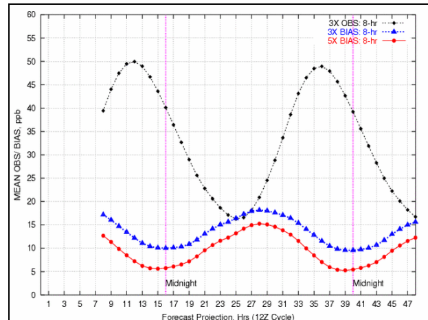
Fig. 3a. Bias, 8 hour 5x3 vs. 3x, August 1 - 15, 2005, 935 stations, 3x mean observations are in black.
