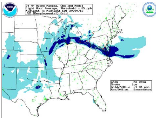
Fig. 5. 8-h spatial map of ozone predictions and observations, 5x model, July 12, 2005.
