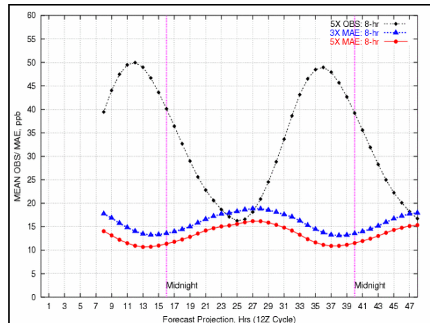
Fig. 3b. MAE, 8 hour 5x3 vs. 3x, August 1 - 15, 2005, 935 stations, 5x mean observations are in black.
