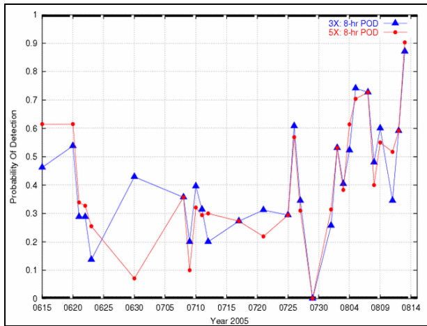
Fig. 2b. 8 hour 5x3 vs. 3x, POD, June 15 – August 13, 2005, 935 stations.
