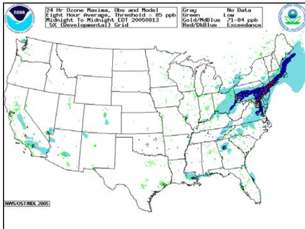
Fig. 4. Spatial map of 8-h ozone predictions with observations, 5x on CONUS grid, August 13, 2005.
