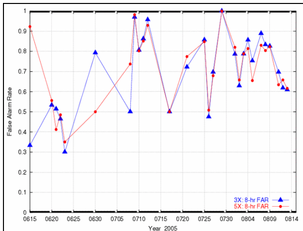
Fig. 2c. 8 hour 5x3 vs. 3x, FAR, June 15 – August 13, 2005, 935 stations.
