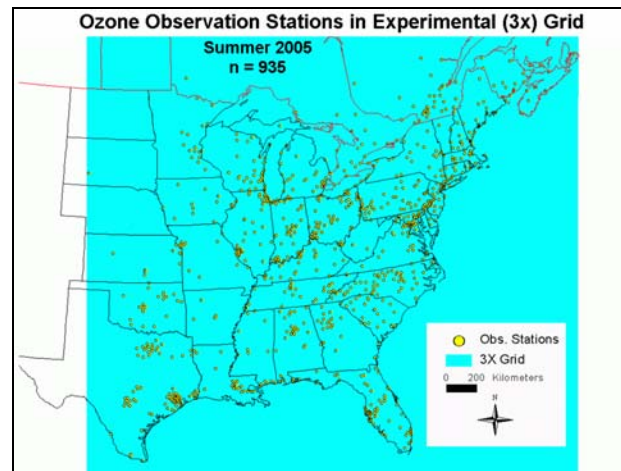
Fig. 1. 3x grid over the eastern U.S., 935 stations, 2005.
