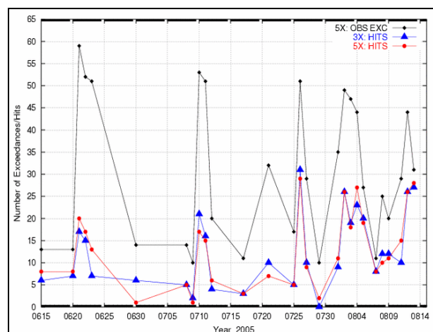
Fig. 2a. 8 hour 5x3 vs. 3x, number of hits, June 15 – August 13, 2005, 935 stations.
